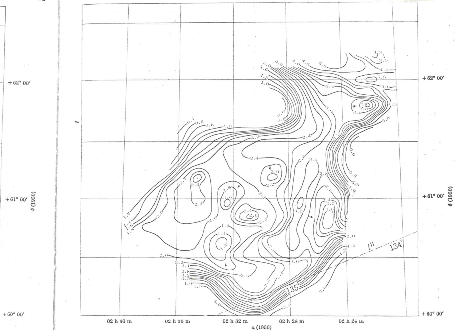
Fig. 4. Interstellar absorption map in magnitude units of IC1795 = W3 and IC1805 = W4 at 46563 Å.
